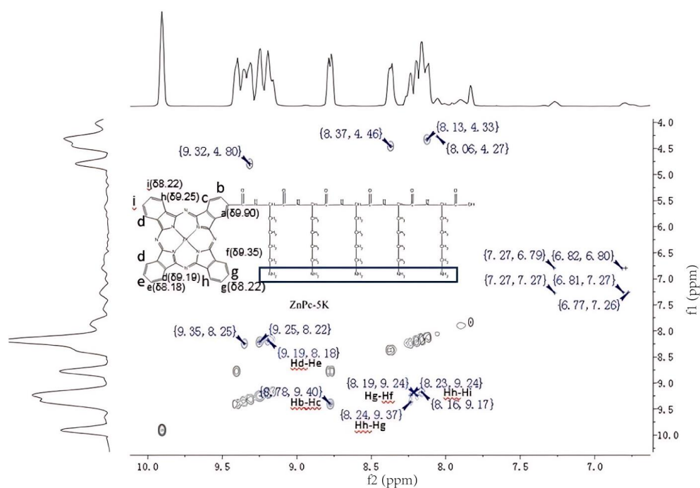
Figure S1. Two-dimensional nuclear magnetic resonance (NMR) spectrum of \text{ZnPc}(\text{Lys})_5 .
