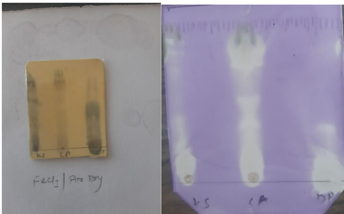
Figure S3. Observation of Phenolic and antioxidant activity using the TLC method.
