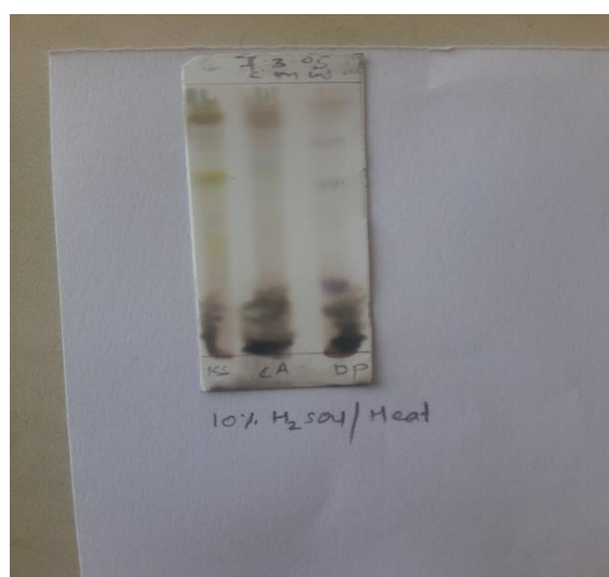
Figure S2. TLC of Drynaria coronans spot (10% H 2 SO 4 /Heat sprayed).
